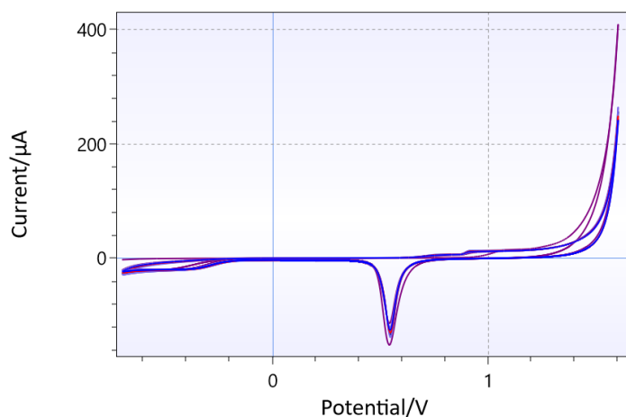
Figure 2 CV, IS-W1-2.C1.RS.35, scan rate 0.1 V/s, E step 5 mV, 1 st , 5 th , 10 th , 15 th , 20 th , 25 th , and 30 th scan
