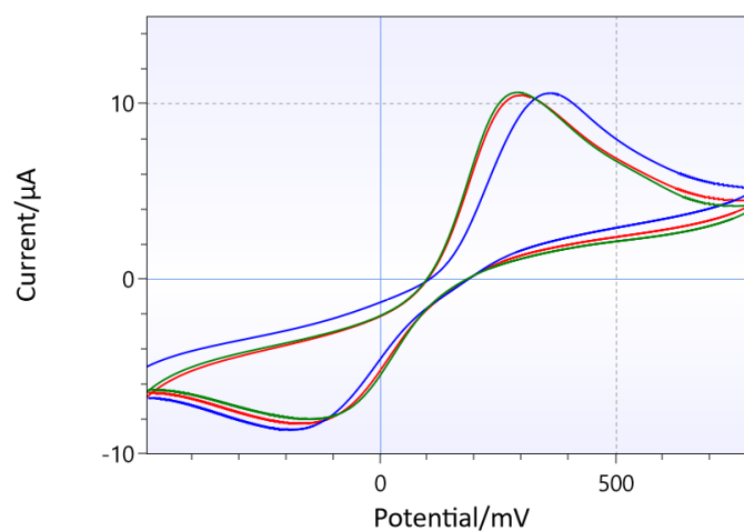
Figure 3 CV, unpolished IS-W1-2.C1.RS.35, scan rate 0.1 V/s, E step 5 mV, 1 st (blue), 2 nd (red), and 3 d (green) scan
