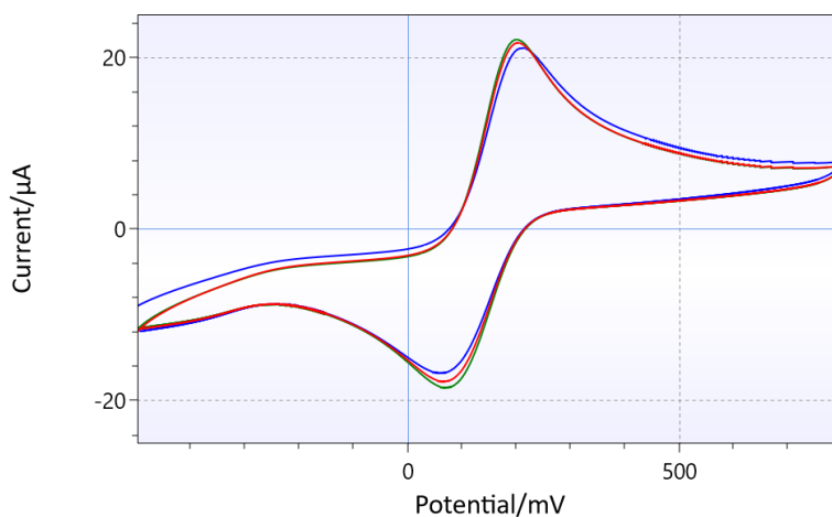
Figure 4 CV, electropolished IS-W1-2.C1.RS.35, scan rate 0.1 V/s, E step 5 mV, 1 st (blue), 2 nd (red), and 3 rd (green) scan
