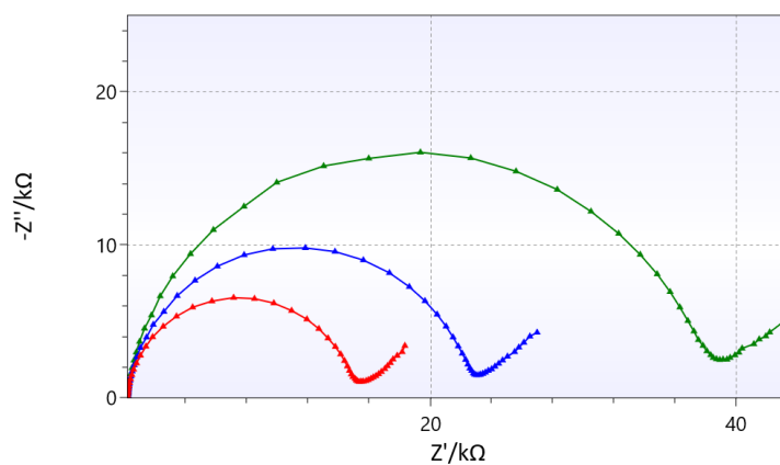
Figure 5 EIS, three unpolished IS-W1-2.C1.RS.35, E dc OCP, E ac 10 mV, frequency range 0.1 Hz to 1 MHz
