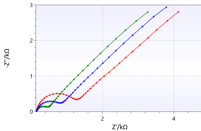
Figure 6 EIS, three polished IS-W1-2.C1.RS.35, E_{dc} OCP, E_{ac} 10 mV, frequency range 0.1 Hz to 1 MHz
