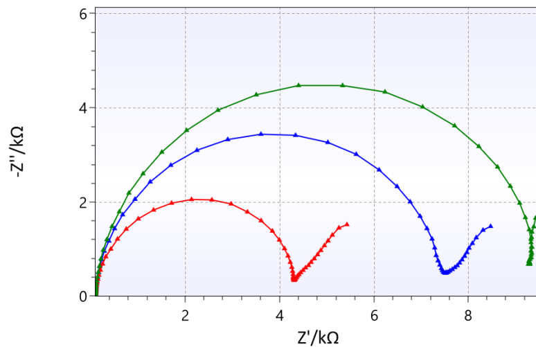
Figure 5 EIS, three unpolished IS-W1-3.C1.RS.50, E dc OCP, E ac 10 mV, frequency range 0.1 Hz to 1 MHz
