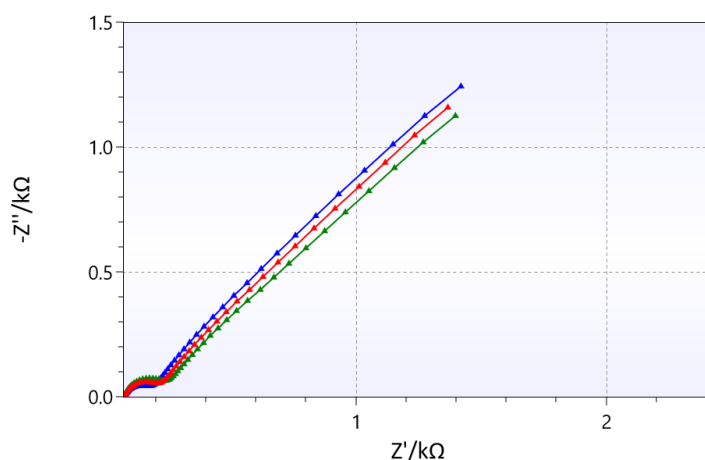
Figure 6 EIS, three polished IS-W1-3.C1.RS.50, E_{dc} OCP, E_{ac} 10 mV, frequency range 0.1 Hz to 1 MHz
