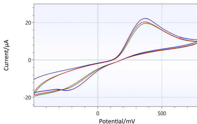
Figure 3 CV, unpolished IS-W1-3.C1.RS.50, scan rate 0.1 V/s, E step 5 mV, 1 st (blue), 2 nd (red), and 3 rd (green) scan
