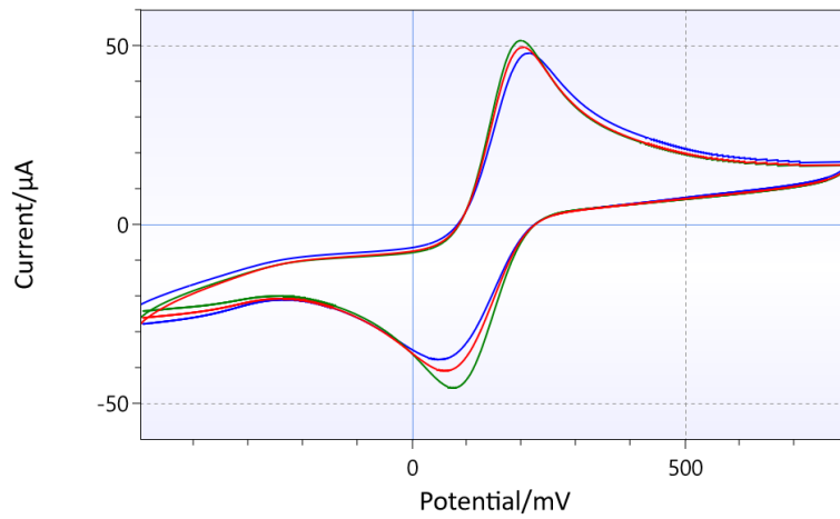
Figure 4 CV, electropolished IS-W1-3.C1.RS.50, scan rate 0.1 V/s, E step 5 mV, 1 st (blue), 2 nd (red), and 3 rd (green) scan
