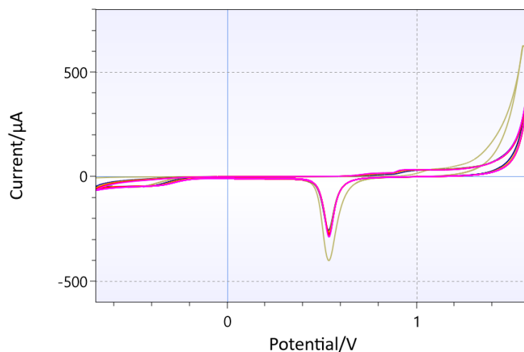
Figure 2 CV, IS-W1-3.C1.RS.50, scan rate 0.1 V/s, E step 5 mV, 1 st , 5 th , 10 th , 15 th , 20 th , 25 th , and 30 th scan
